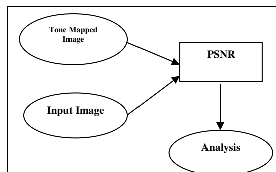
Figure. 6. Analysis
