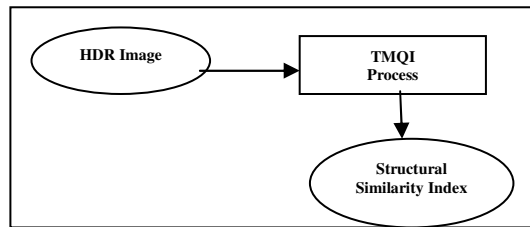
Figure. 3. TMQI Process
