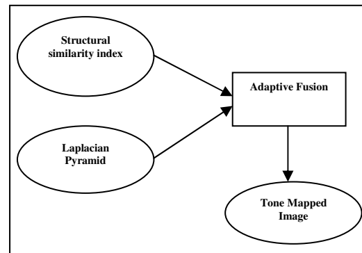
Figure. 5. Adaptive Process
