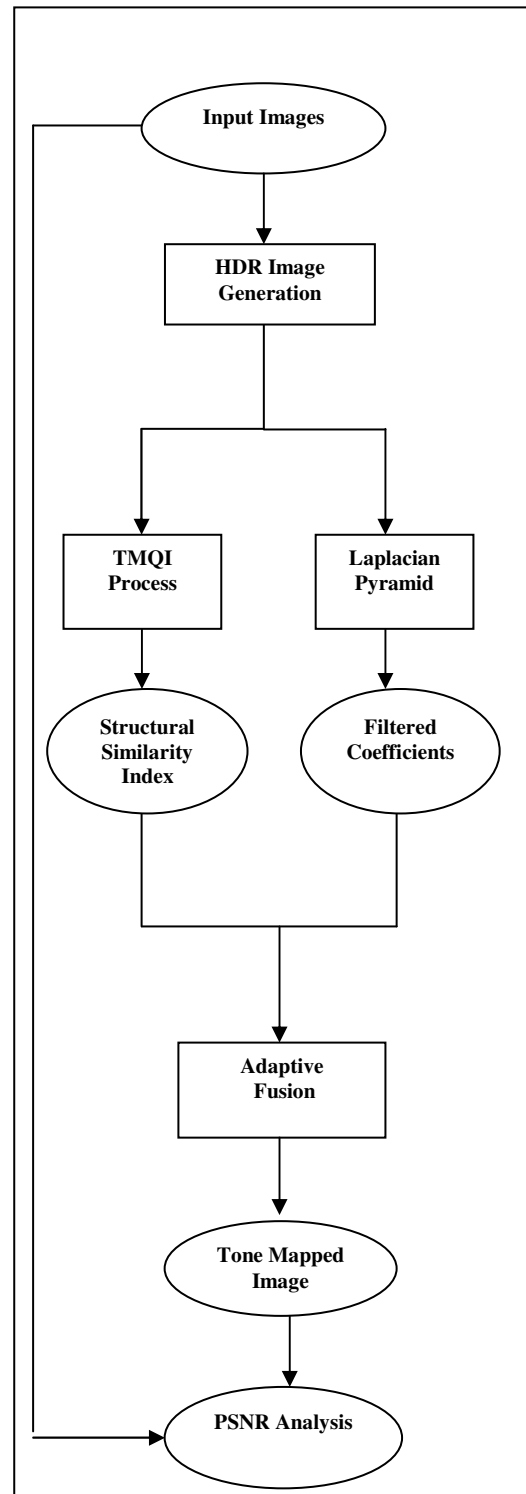
Figure.2. Flow chart
