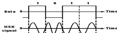
Figure-2 Signal Using MSK Modulation
