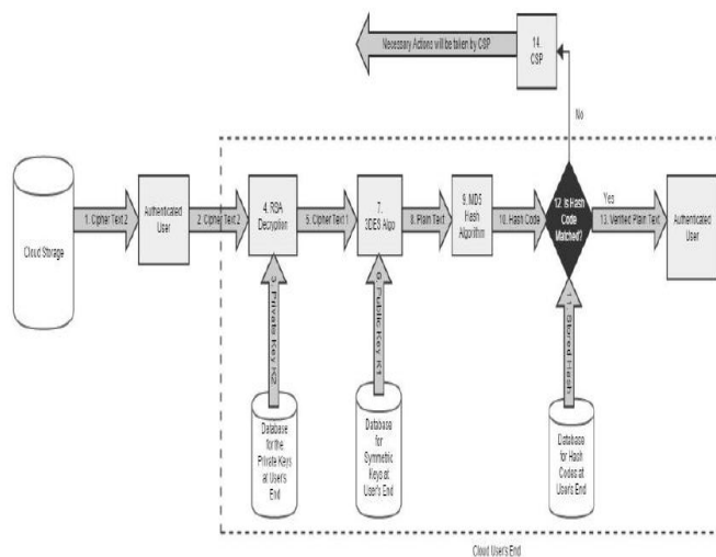
Figure 6. Information Recovery and Assurance of Authenticity
