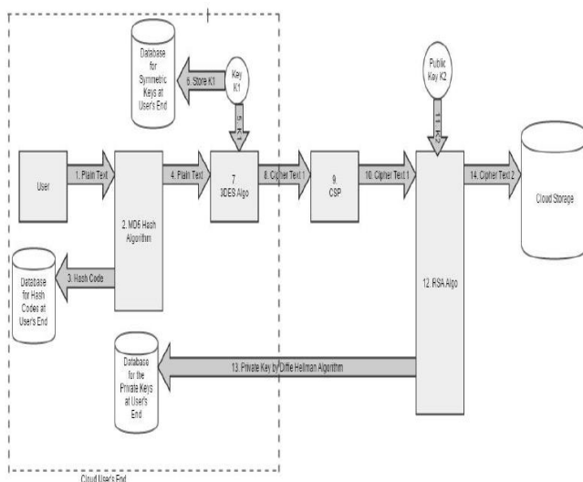
Figure 4. Data Storage on cloud
