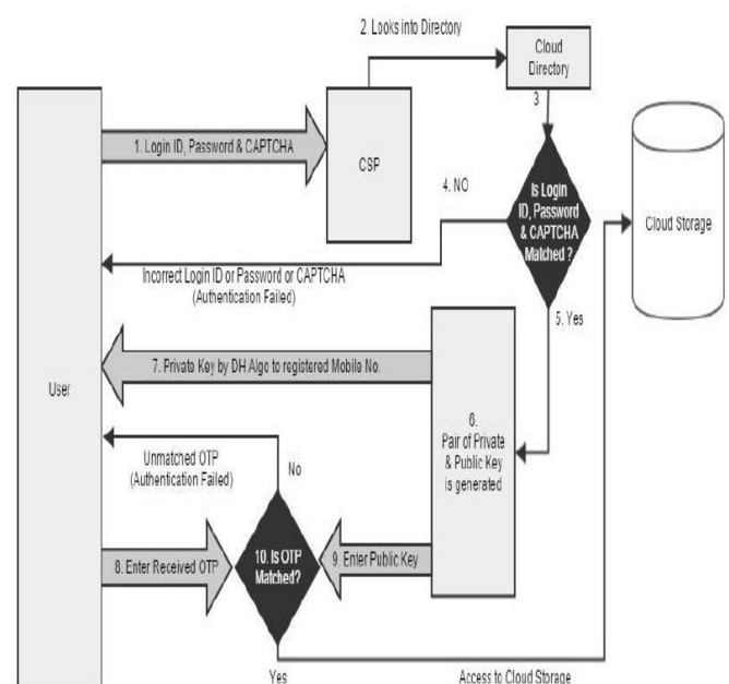
Figure 5. Authorization of the Data Requester
