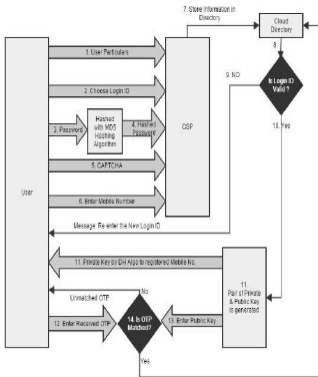
Figure 3. Cloud User Registration
