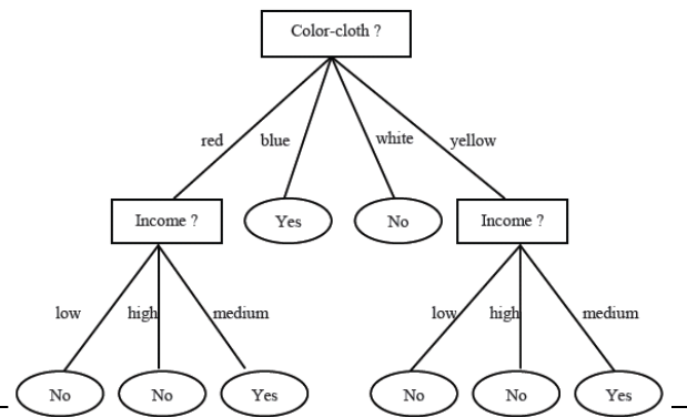
Figure (a). The obtained decision tree using ID3 algorithm
