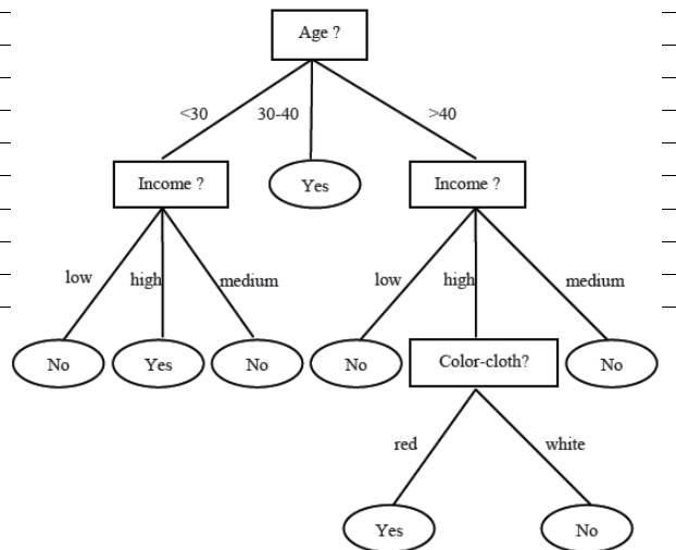
Figure (b). The obtained decision tree using improved ID3 algorithm
