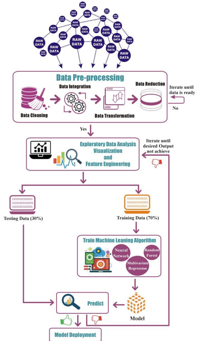
Figure 2: Train delay prediction System using Machine learning.
