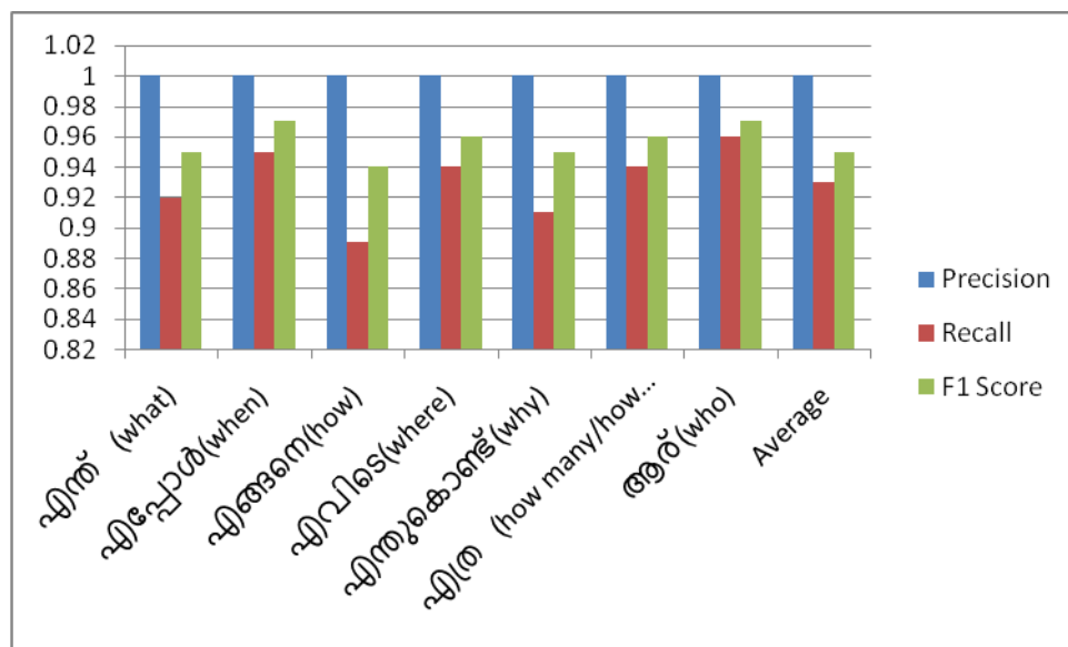
Figure 2: Graphical Performance Evaluation for SVM
