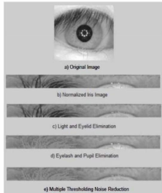
Figure 2.4: Example of application of the proposed method against an iris image corrupted with strong eyelash pixels [2]
