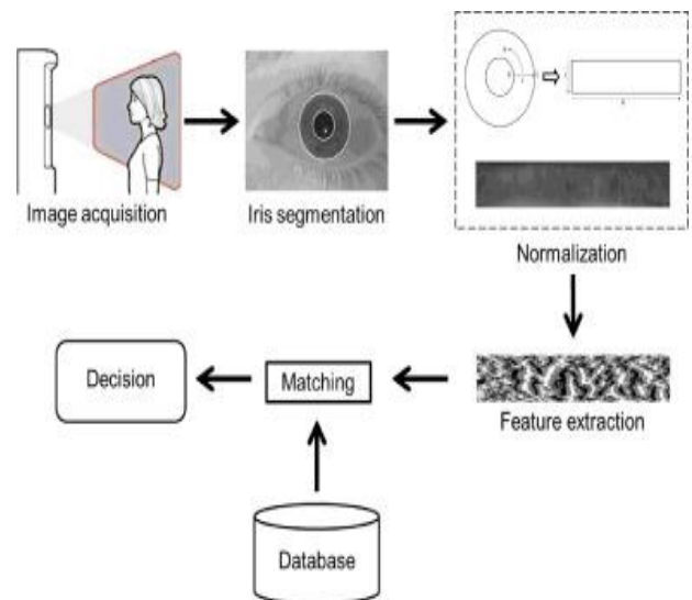
Figure 1.5: Iris Recognition Process [11]
