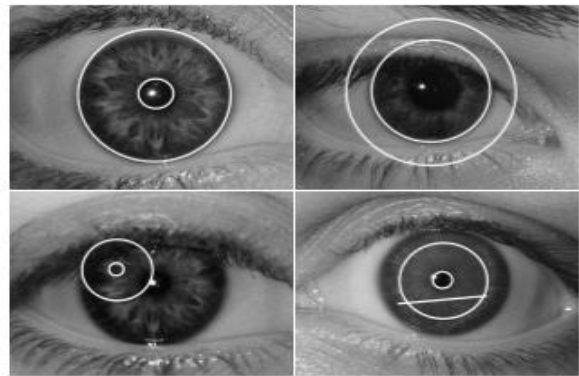
Figure 2.8: Results of the Iris Localization performed by MIRLIN algorithm. Correctly localized iris is in 1st image. Other three images present irides that were incorrectly localized. [6]
