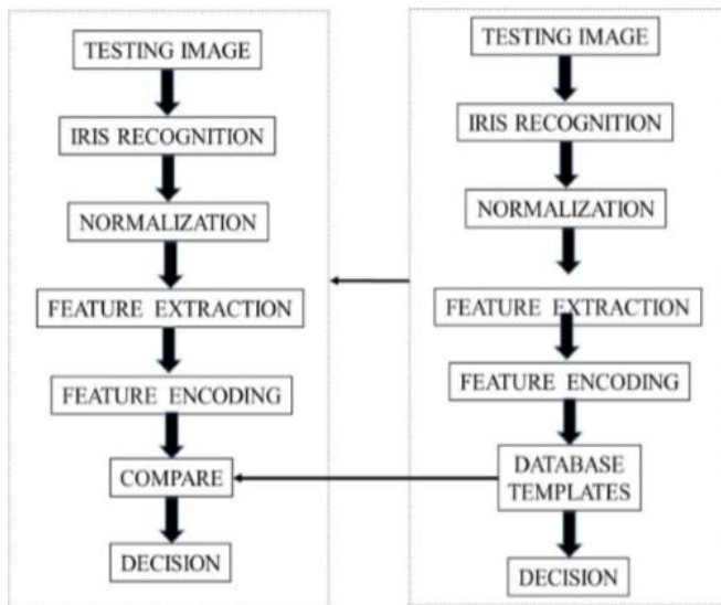
Figure 2.9: Flow of Proposed Method of Iris Detection [8]
