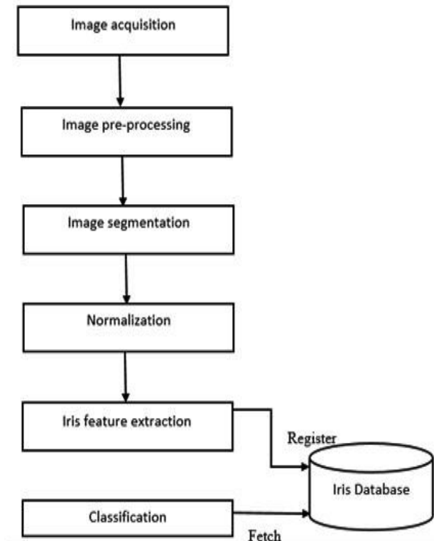
Figure 1.4: Typical Iris Recognition Process [12]
